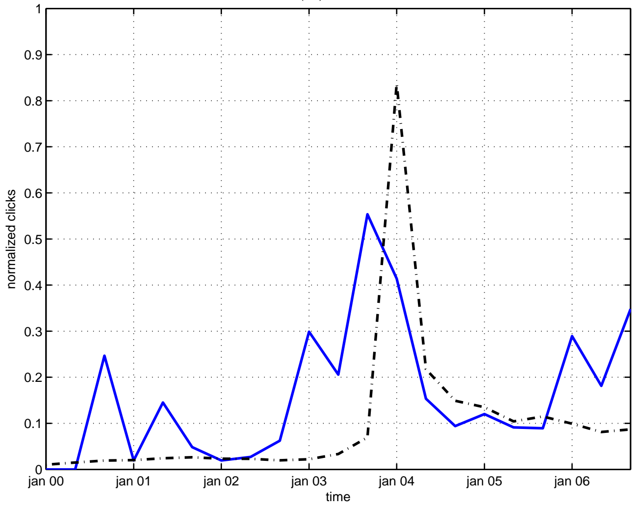
sl(2,r) invariance
