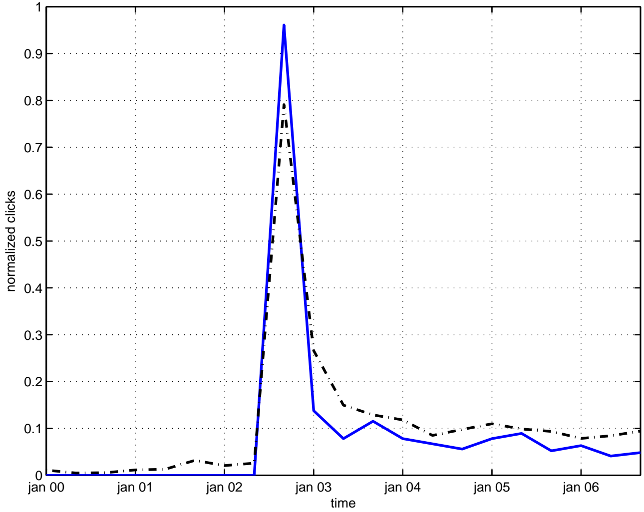
sl(2,r) gauge field theory
