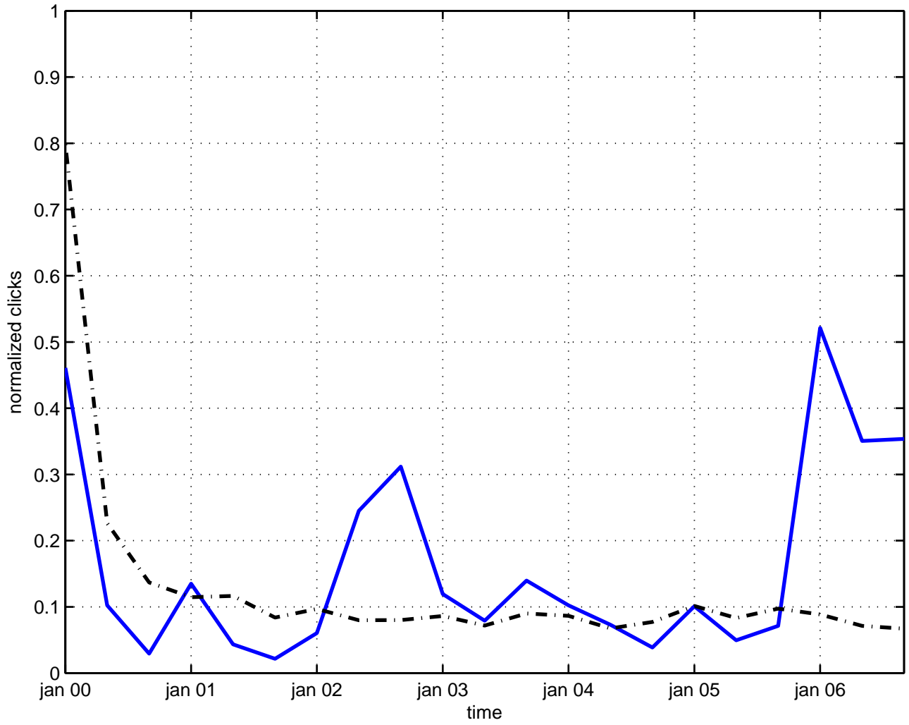
sl(2,r) algebra
