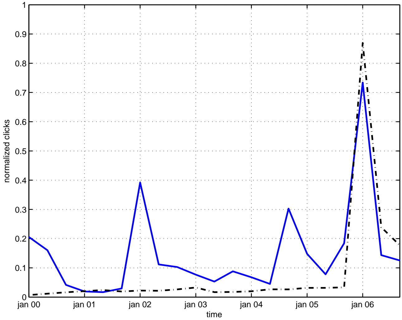
sl(2,c) symmetry
