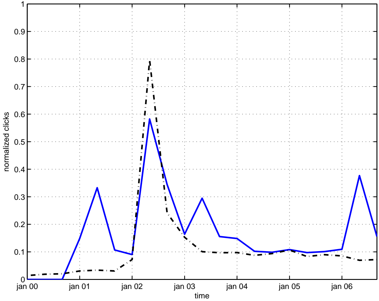
sl(2,c) invariance
