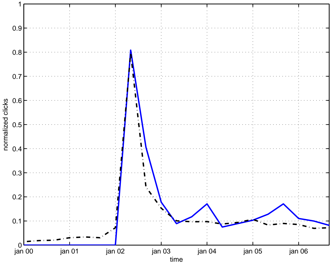
sl(10) group theory
