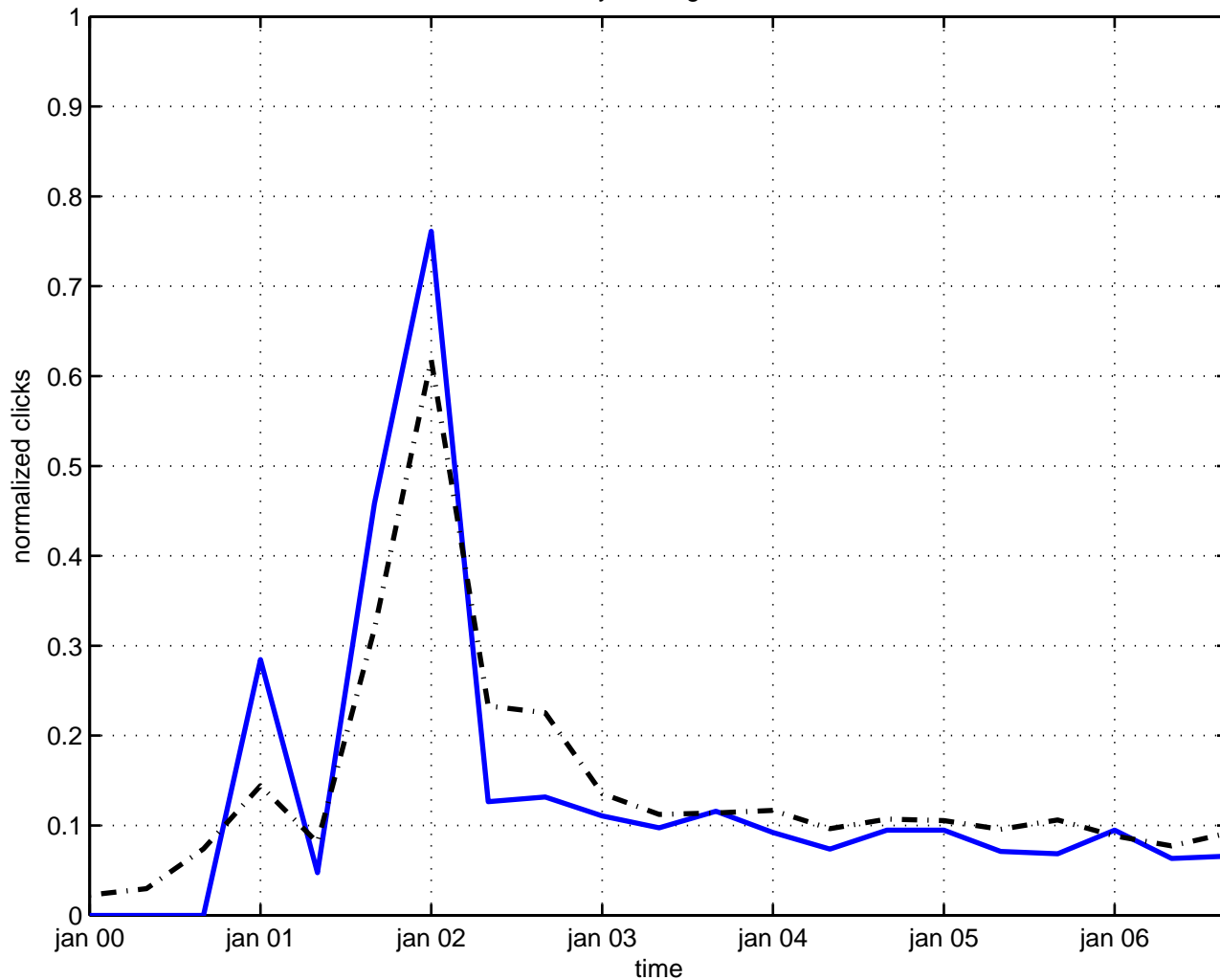
sklyanin algebra
