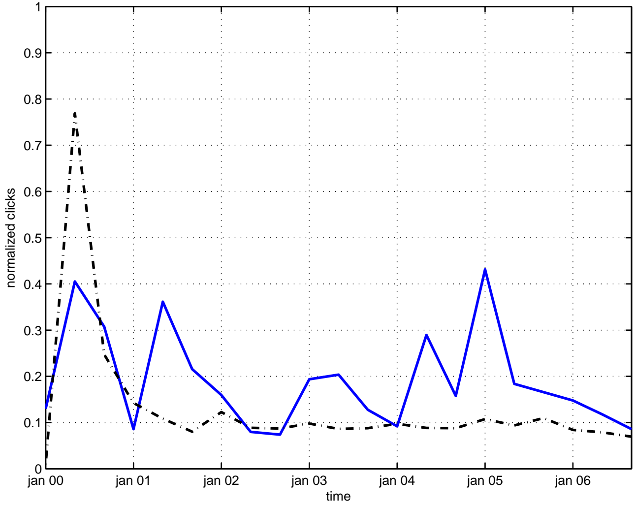
sinh-gordon model
