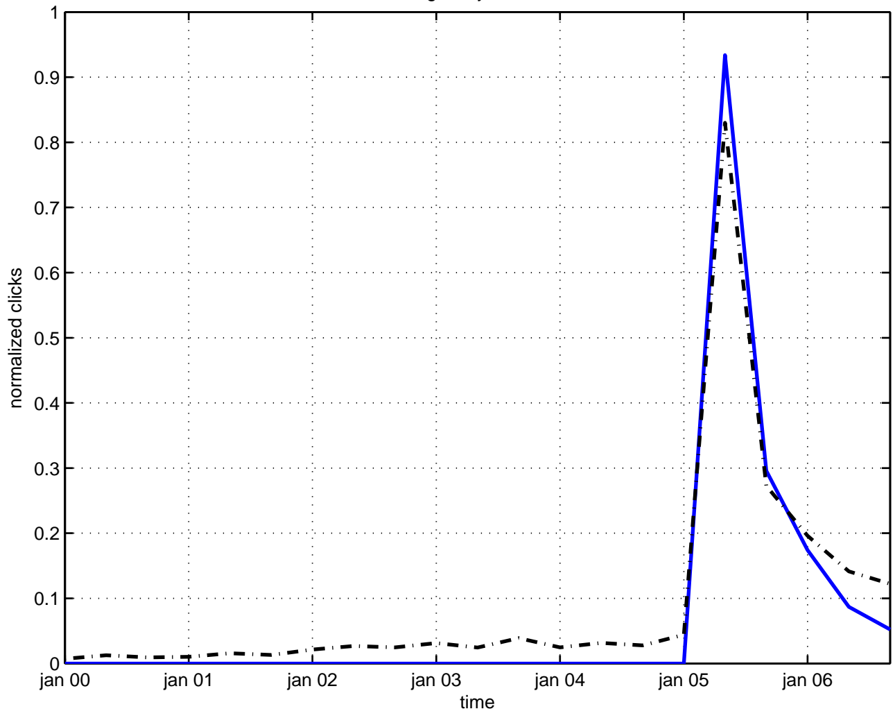
singularity surface
