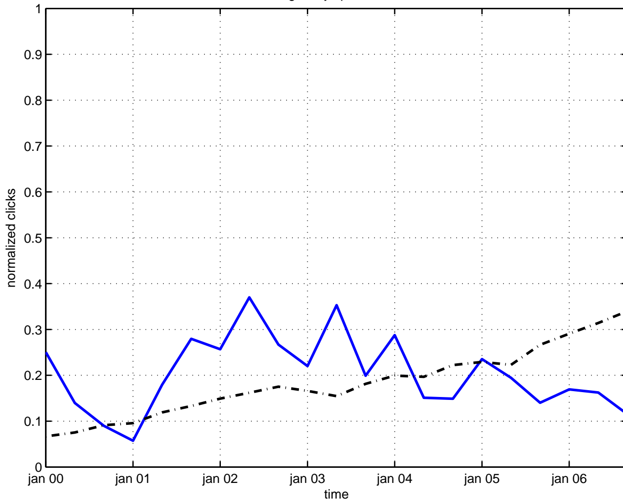
singularity space-time
