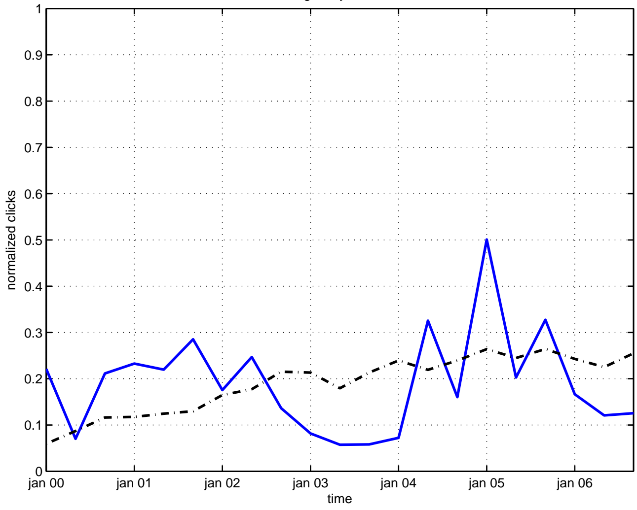
singularity orbifold
