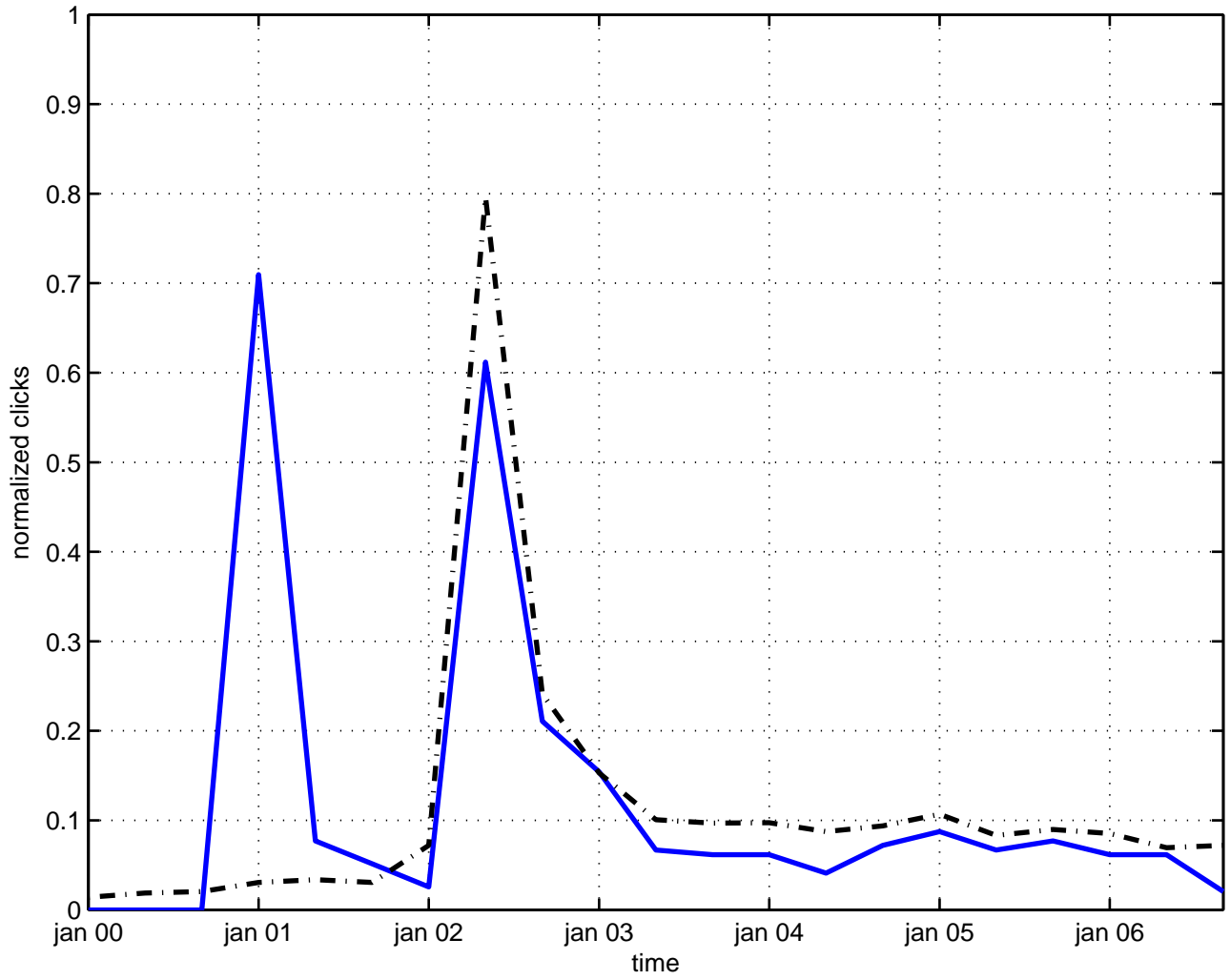
singularity membrane model
