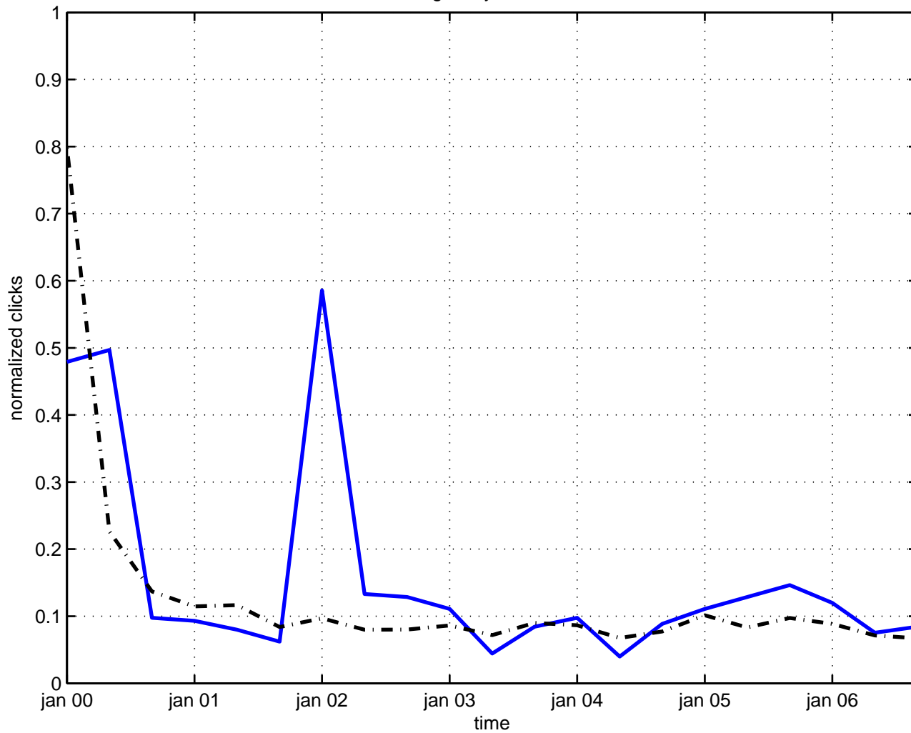
singularity instanton
