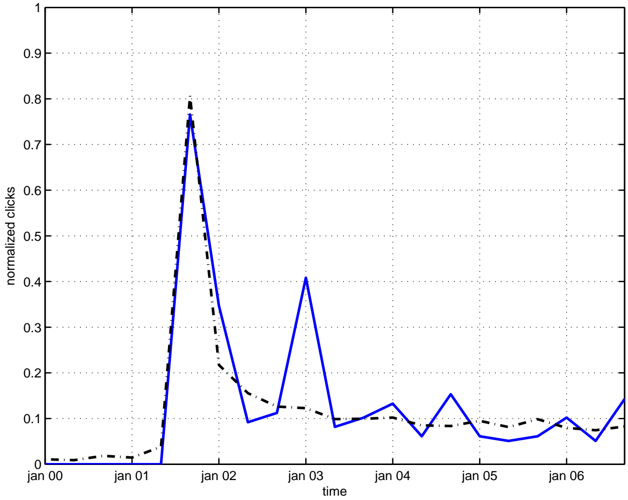
singularity horizon
