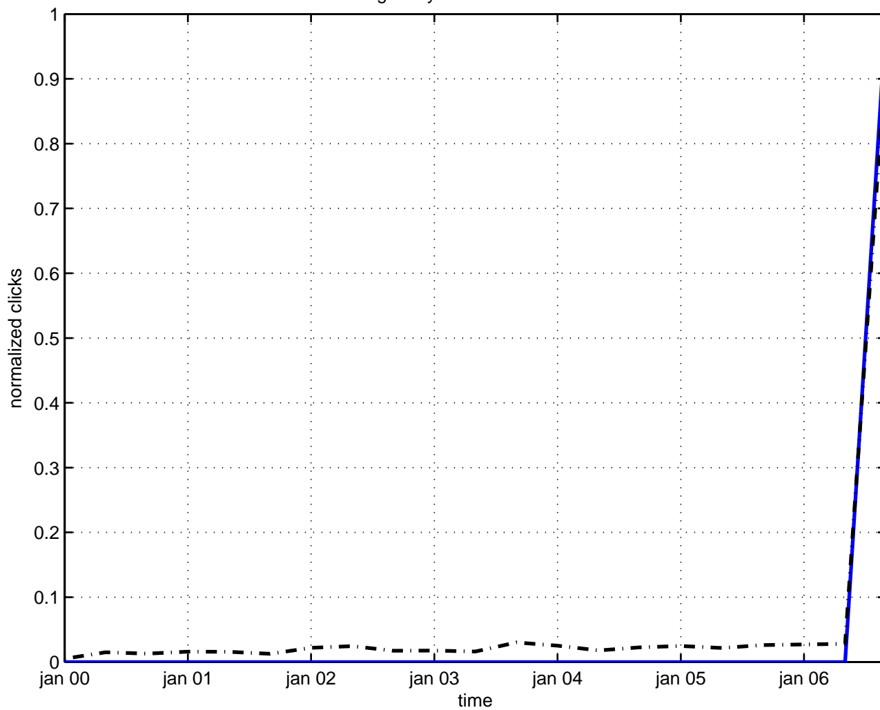
singularity correlation function
