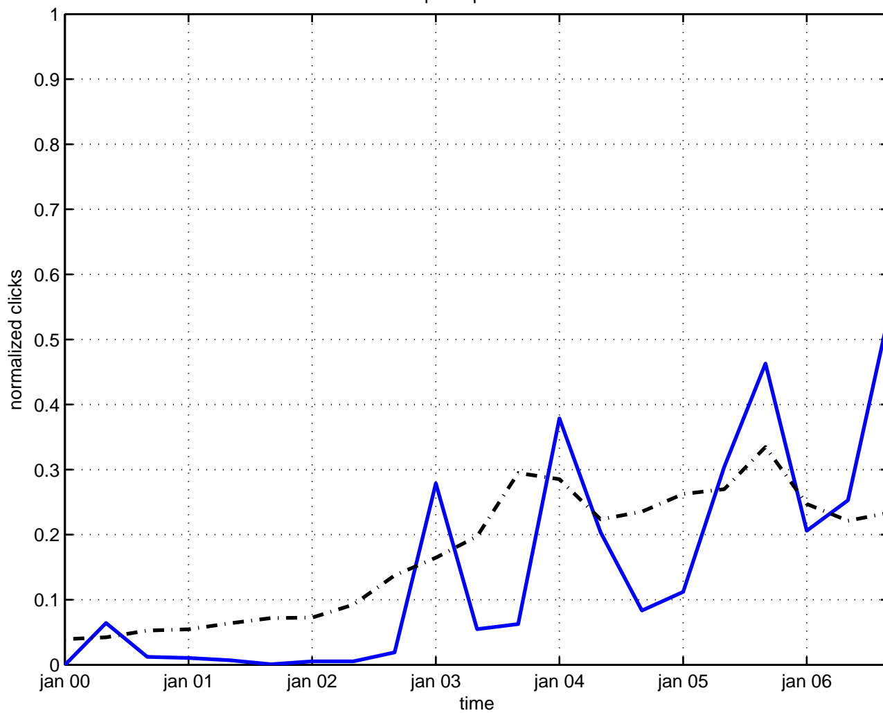
simplex space-time
