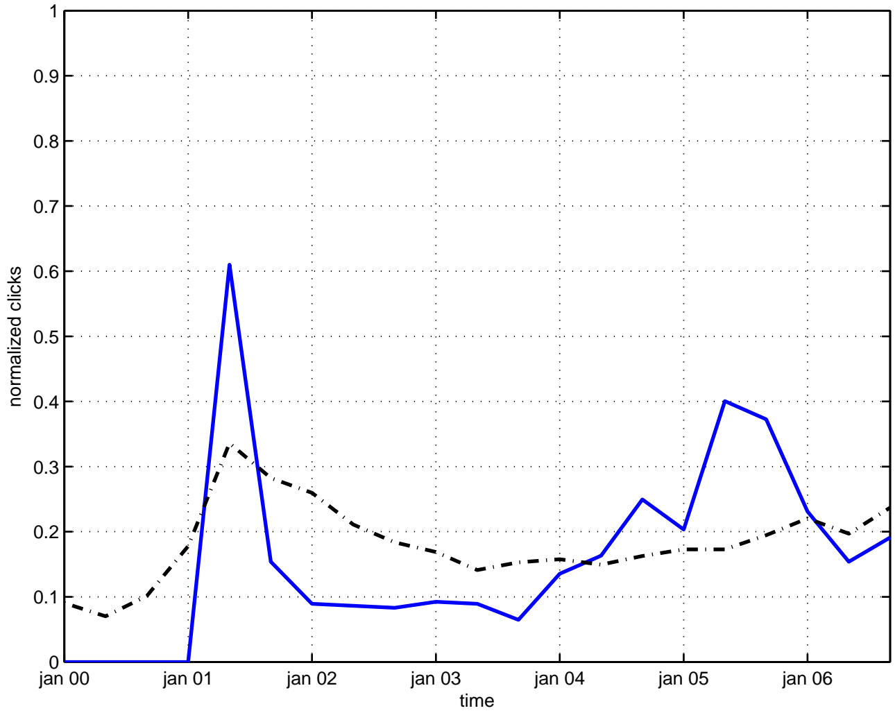
simplex regularization
