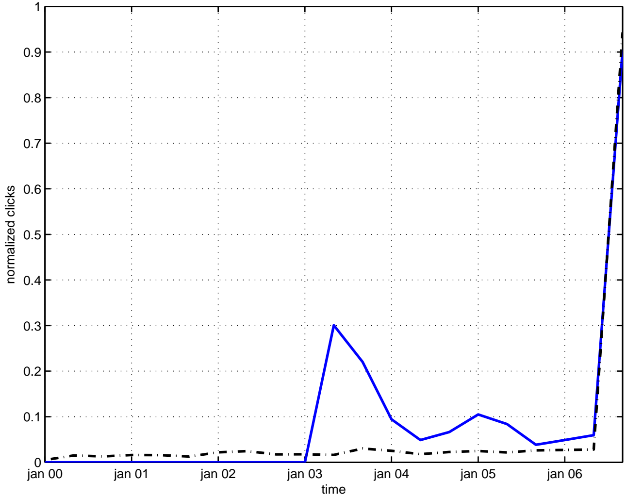
simplex quantum gravity
