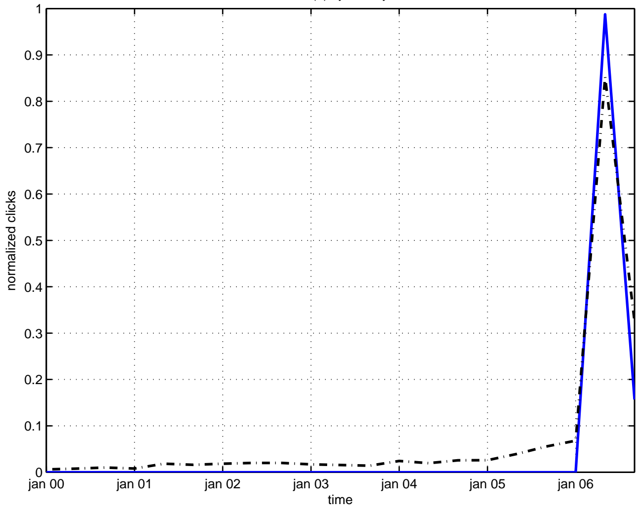
sim(2) symmetry
