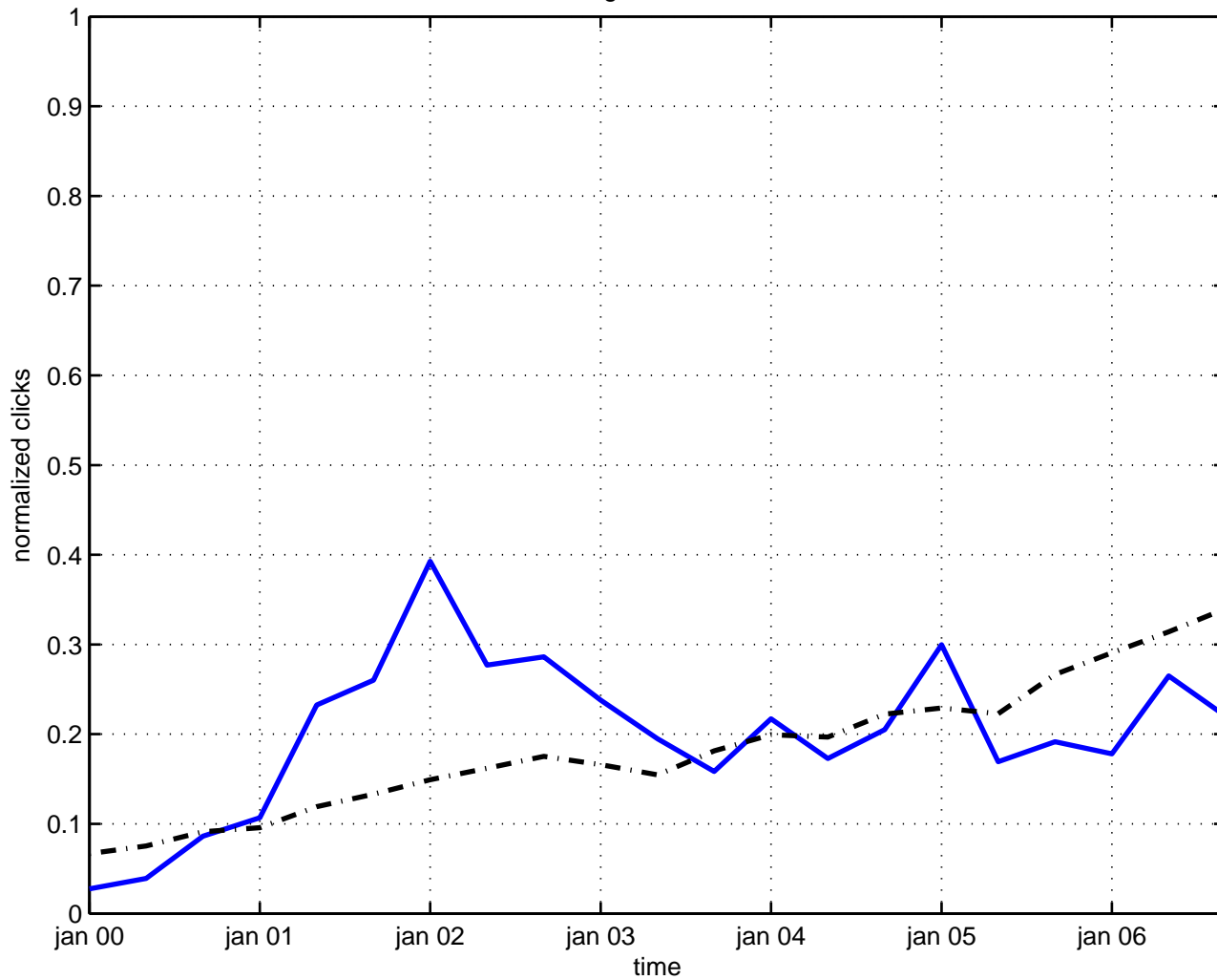
sigma model
