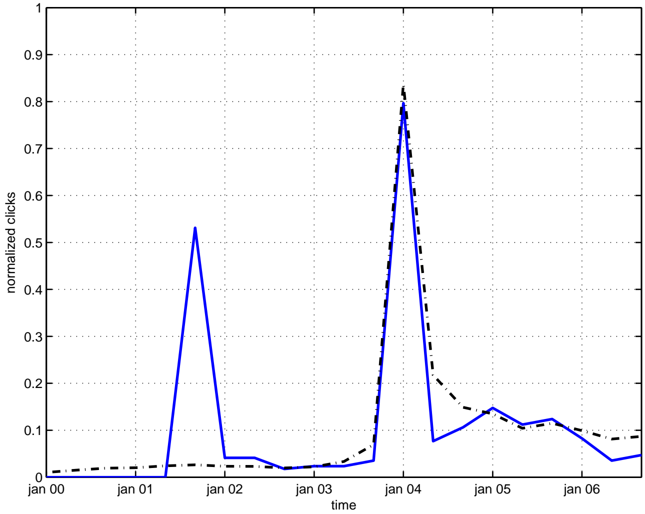
short-range interaction
