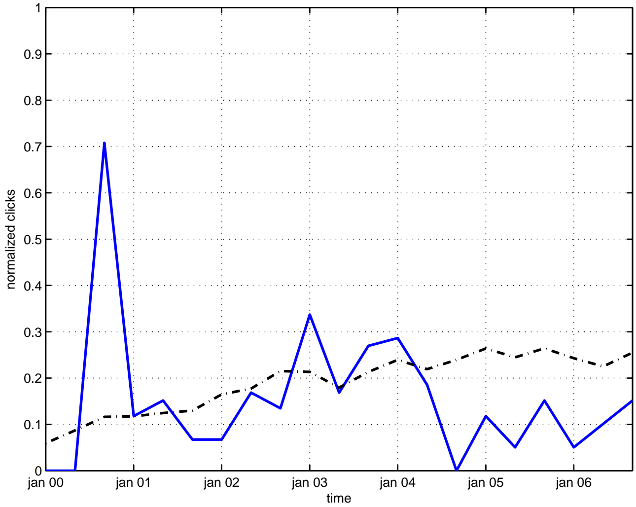
short-range correlation
