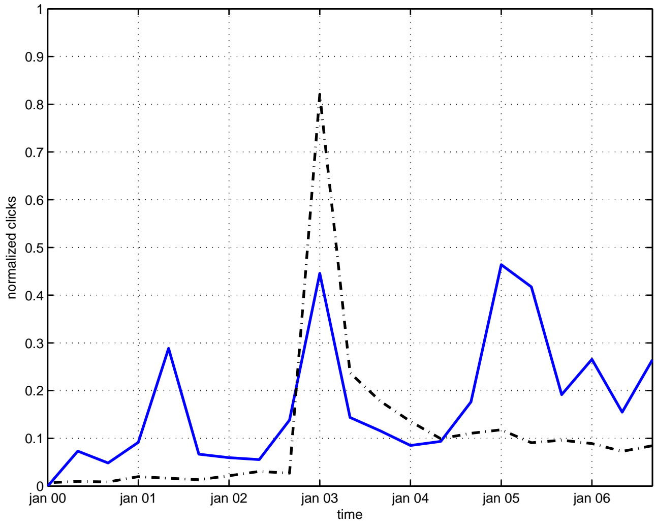
shock waves
