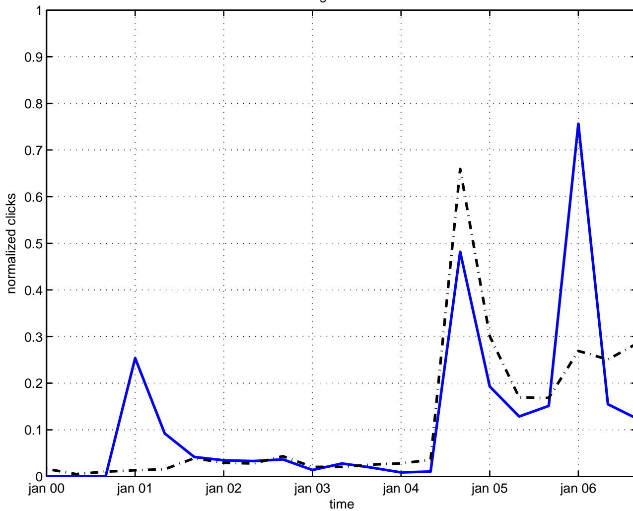
shock waves gravitational radiation
