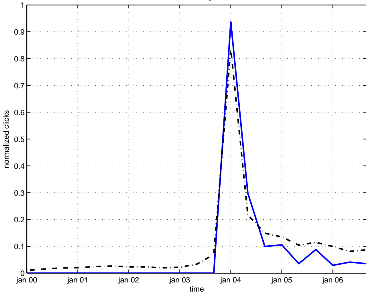
shock waves background field
