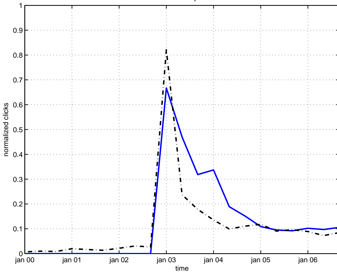
set theory
