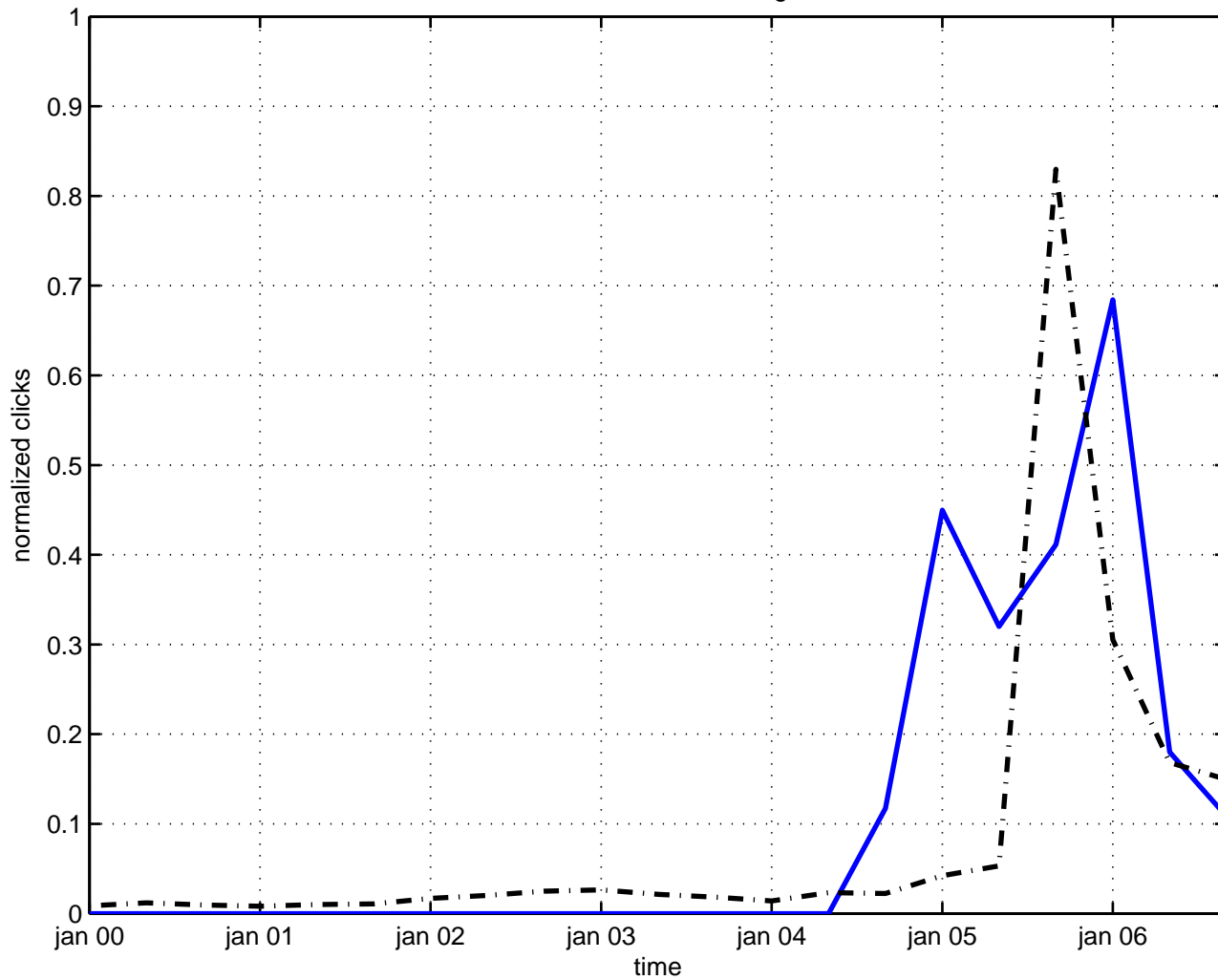
semiclassical tunneling
