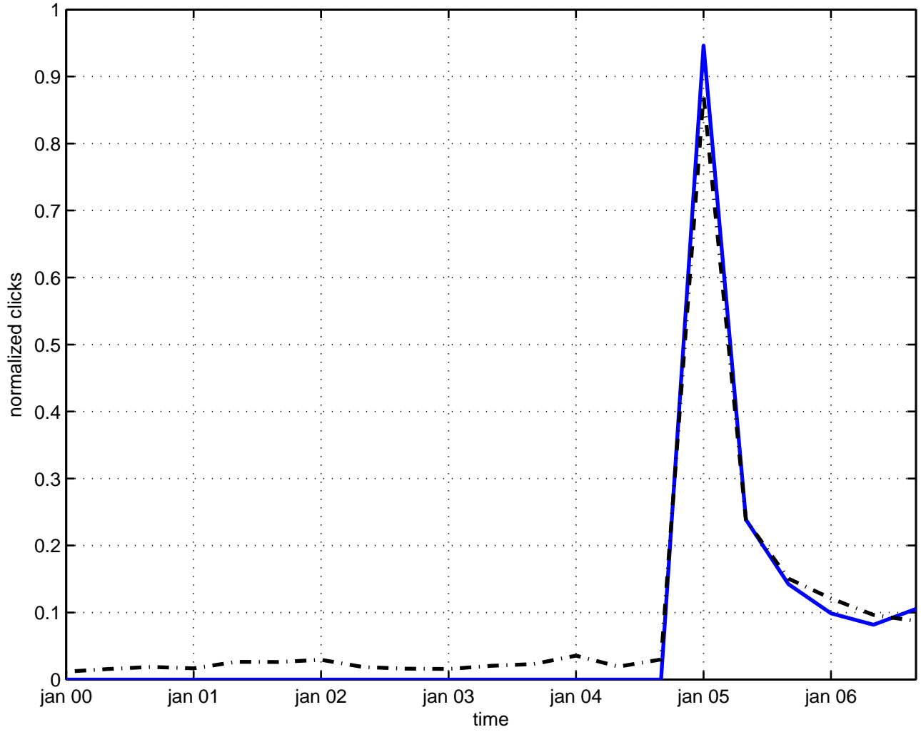
semiclassical quantum gravity
