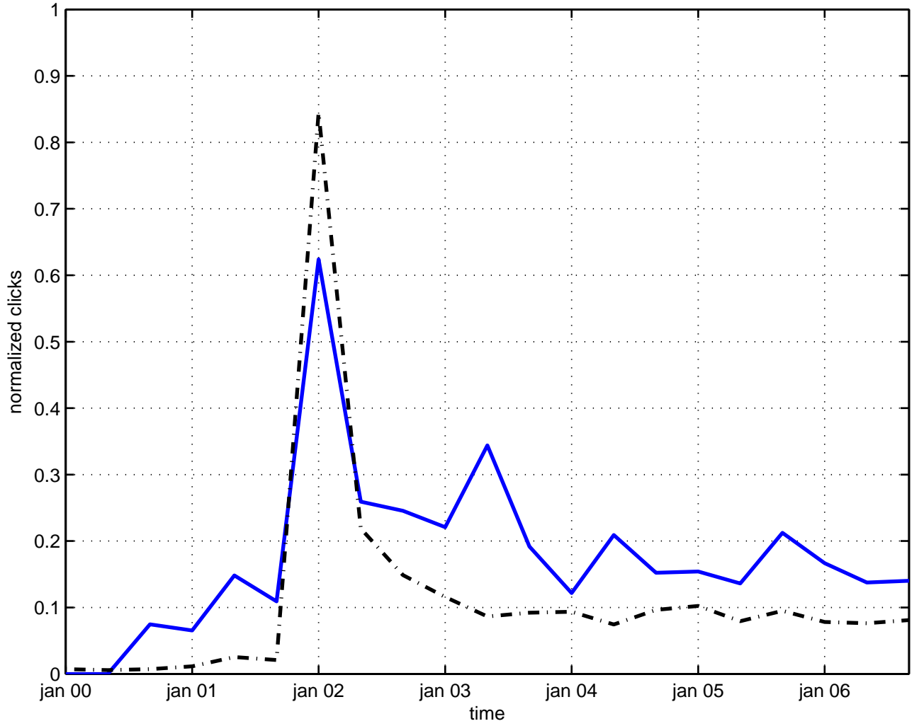
semiclassical quantization
