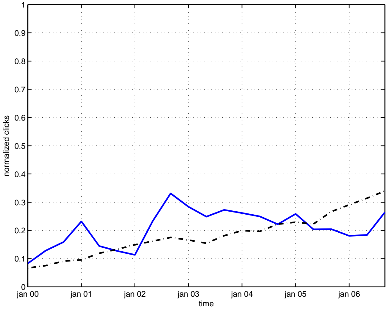
seiberg-witten model
