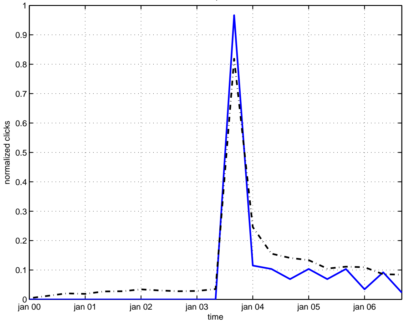
sea quark
