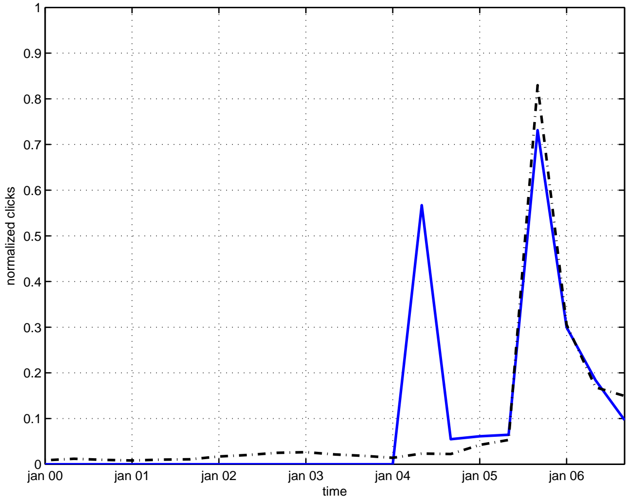
screening potential
