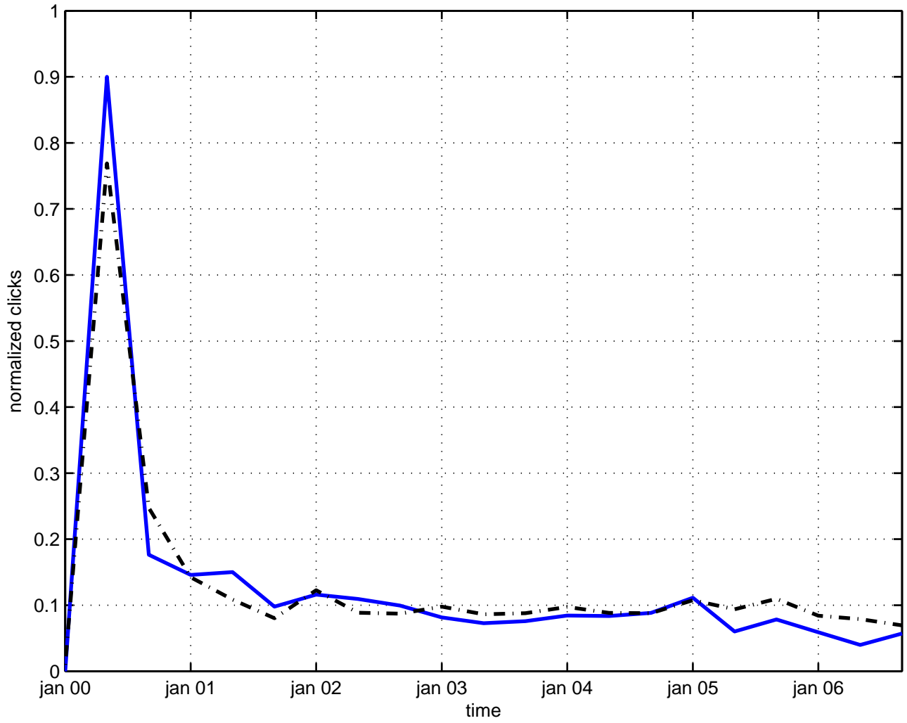
screening effect
