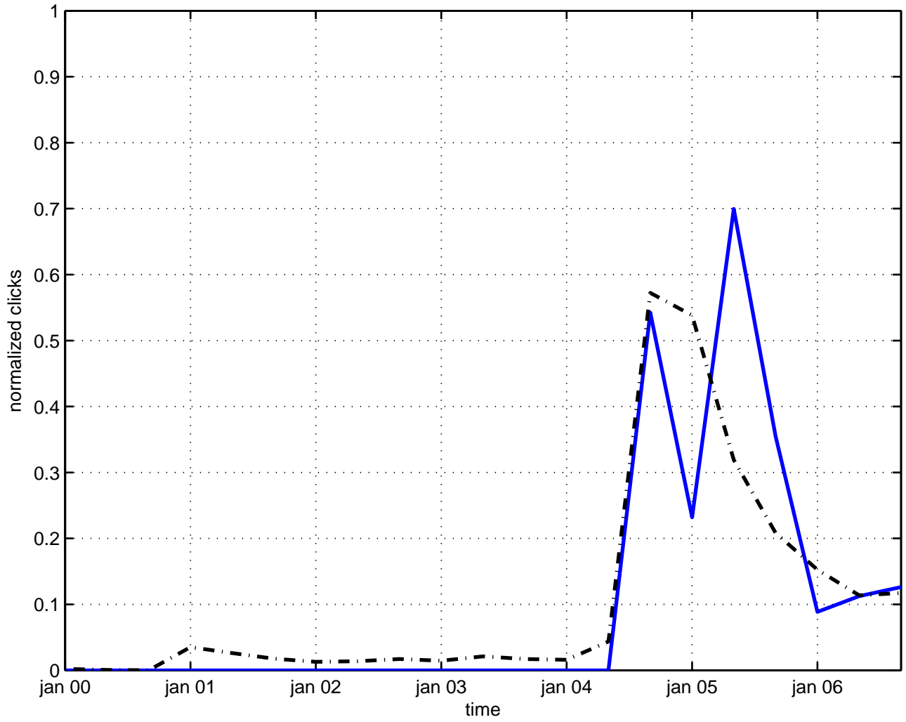
schwarzschild background
