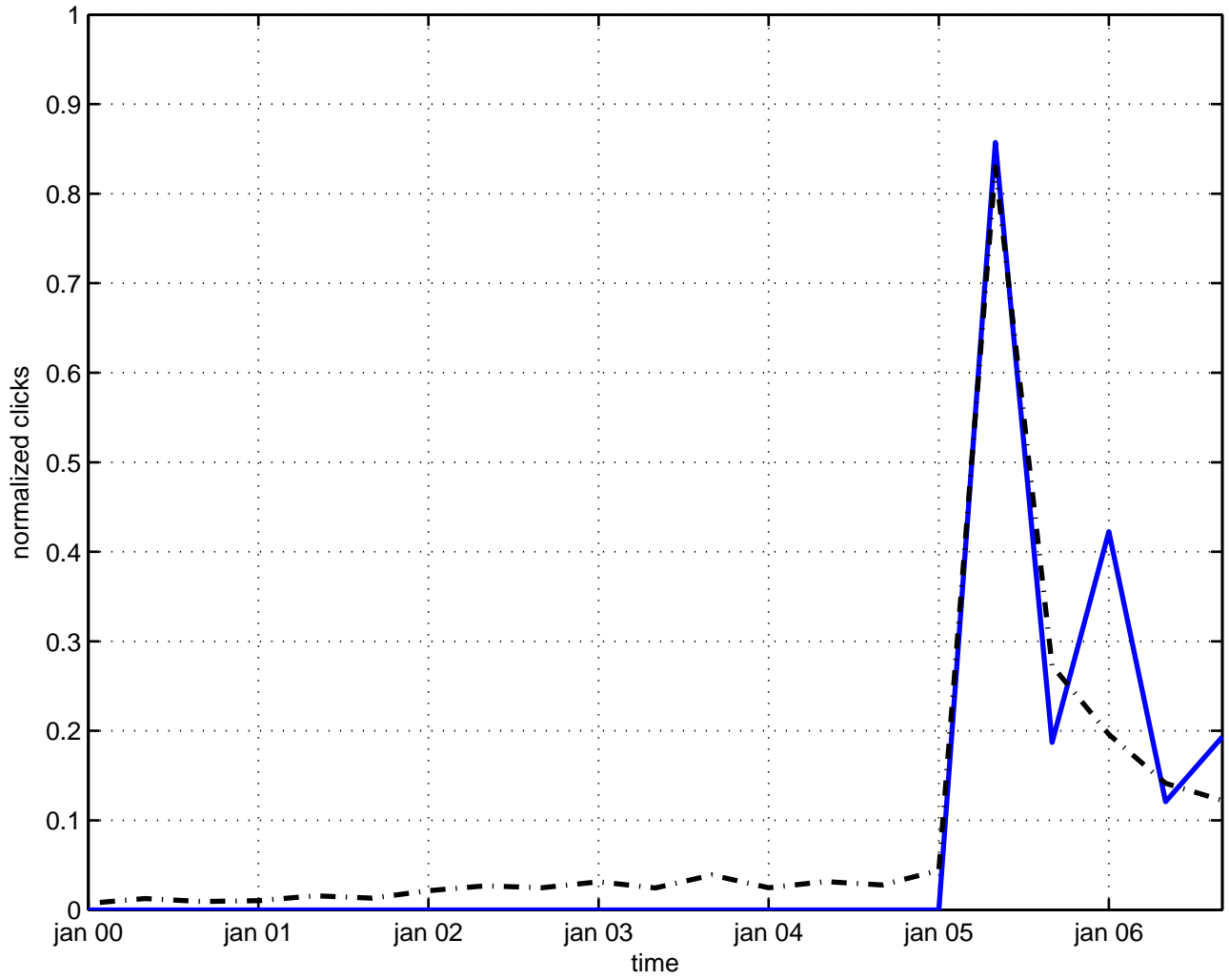
schroedinger terms current algebra
