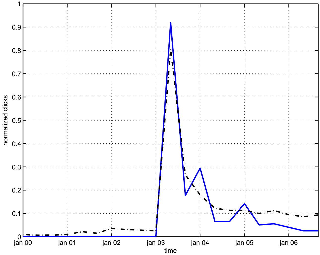
schroedinger operator
