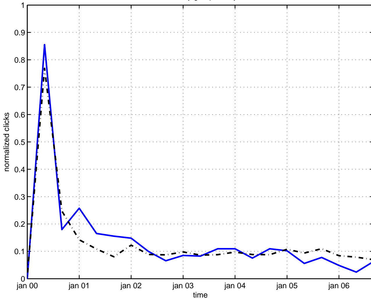
schottky group theory
