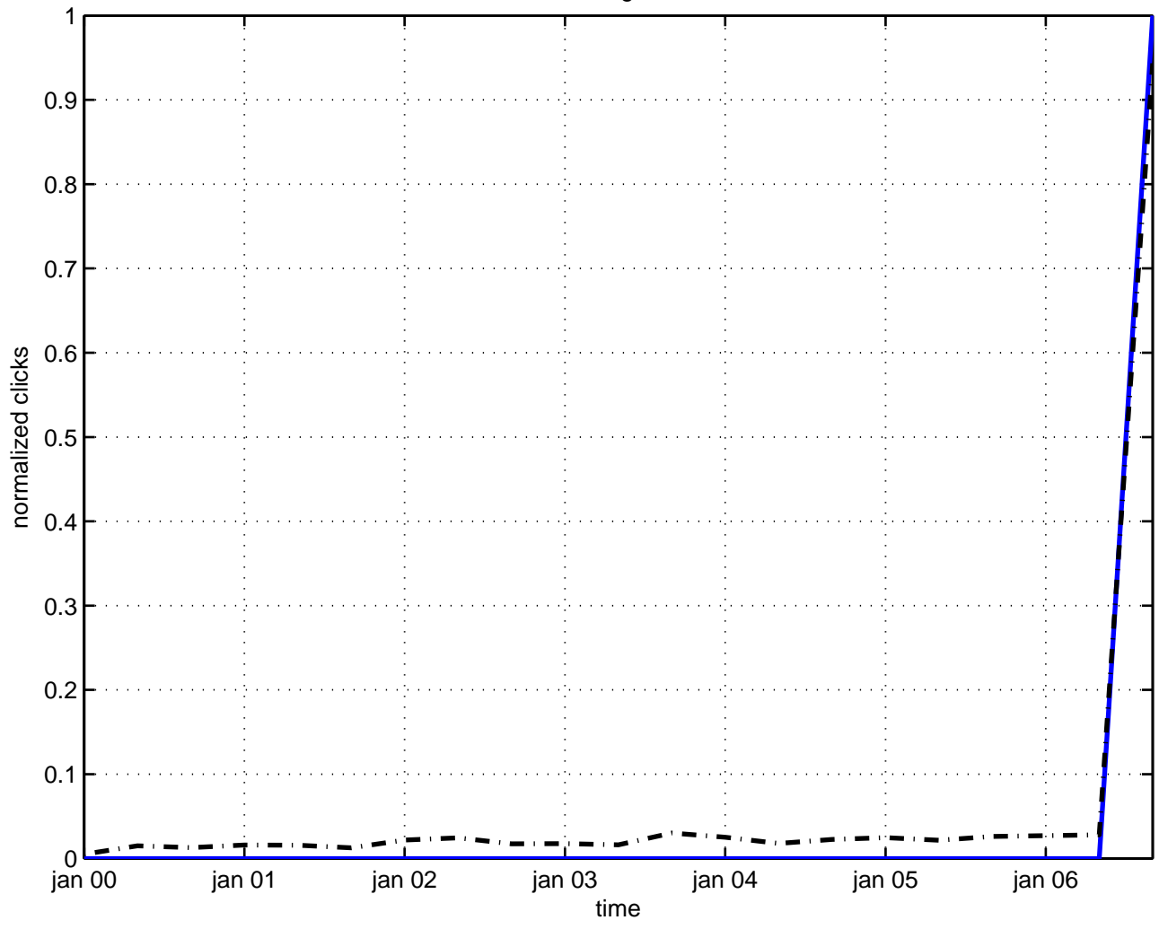
scattering vortex
