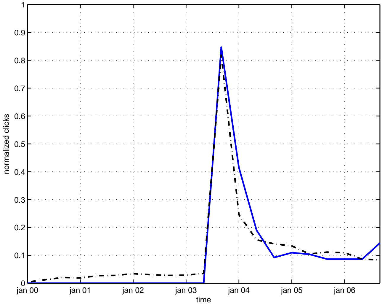
scattering photon photon
