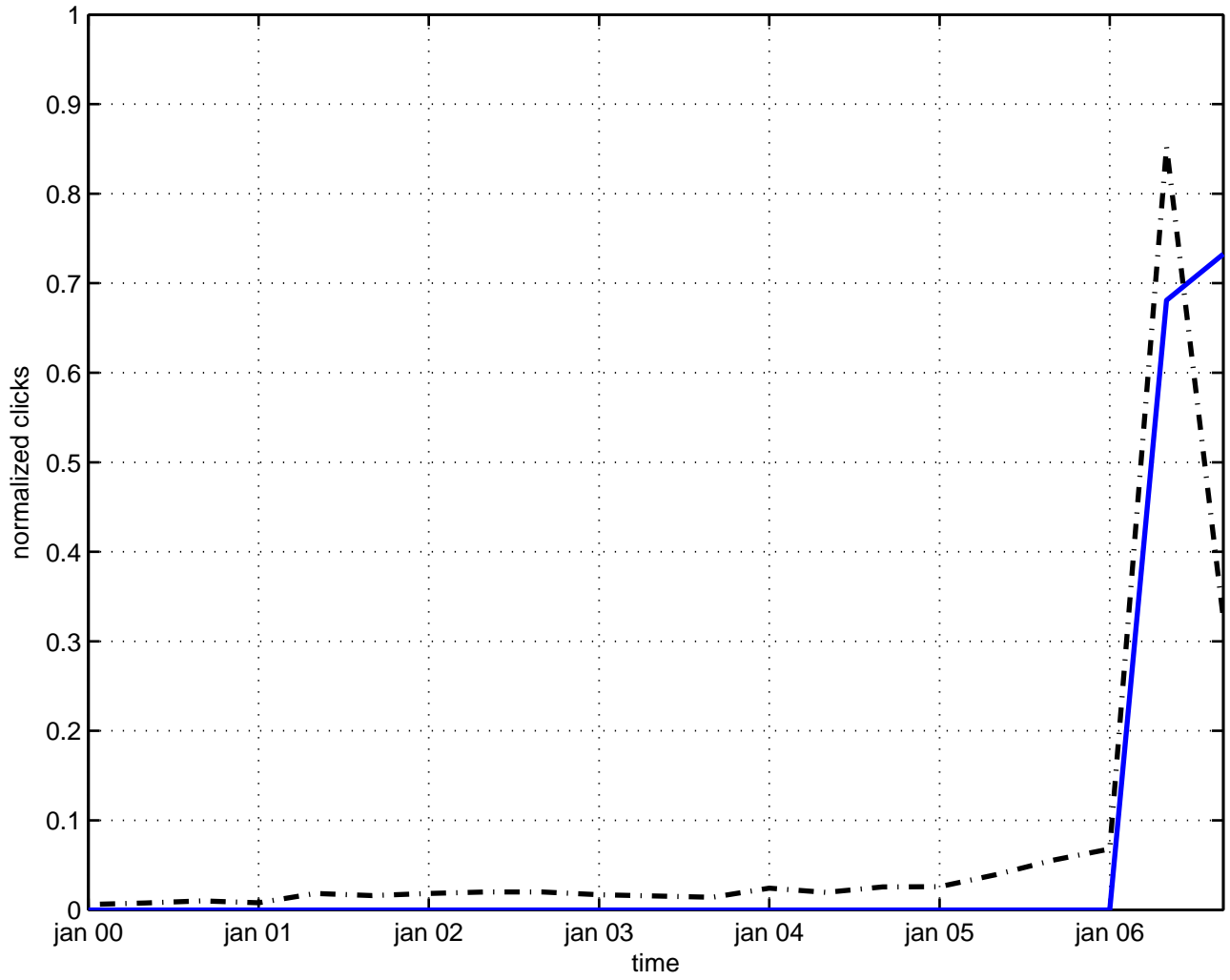
scattering magnon
