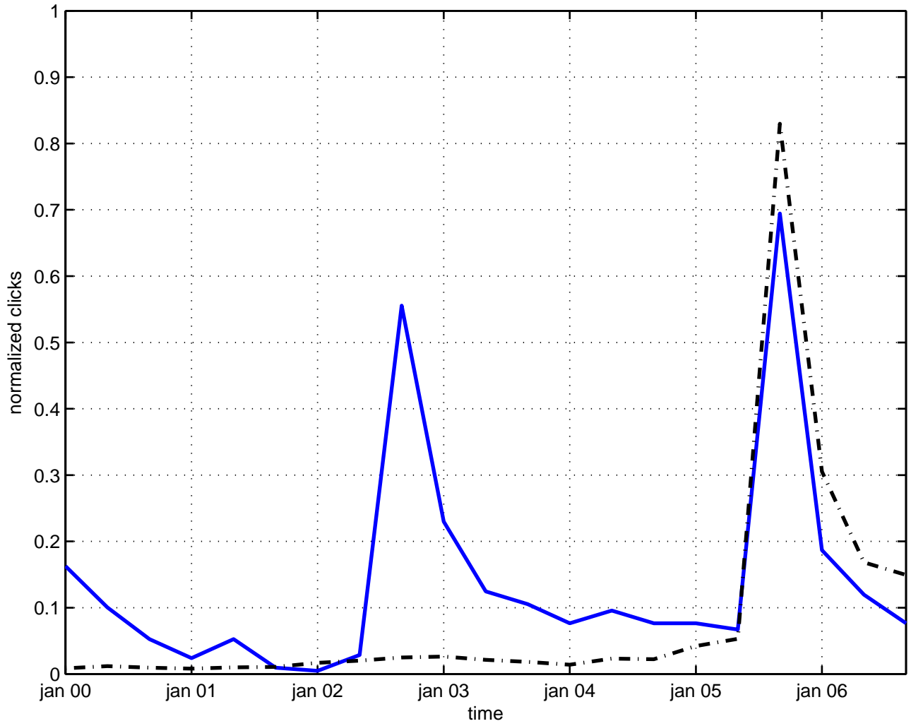
scattering magnetic monopole
