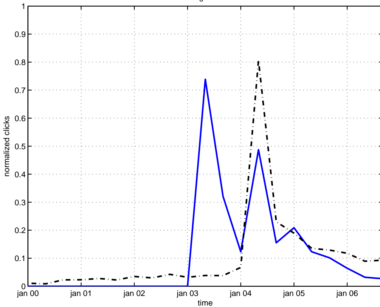
scattering black hole
