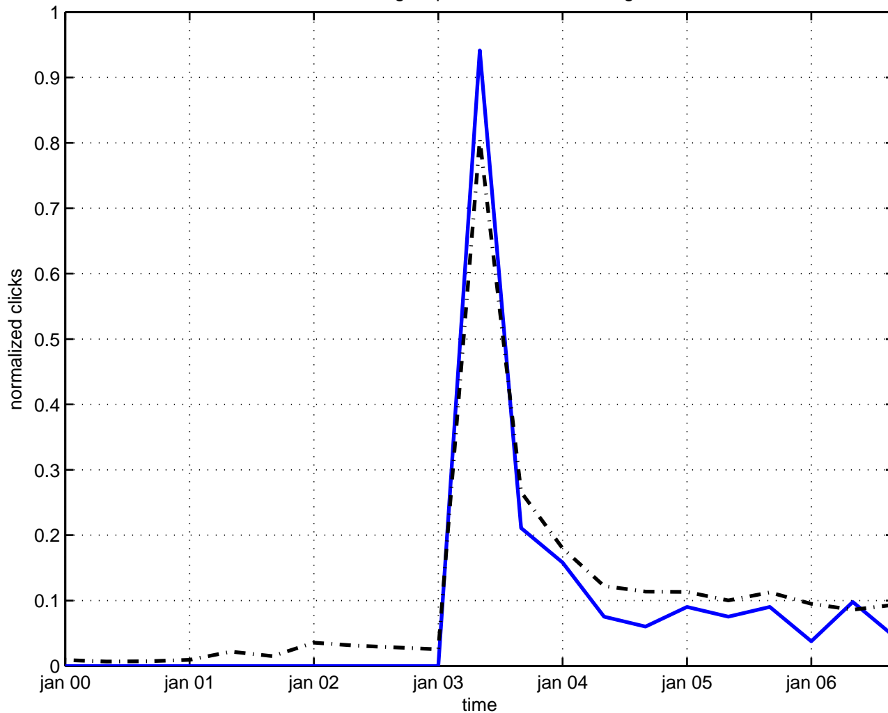
scattering amplitude elastic scattering
