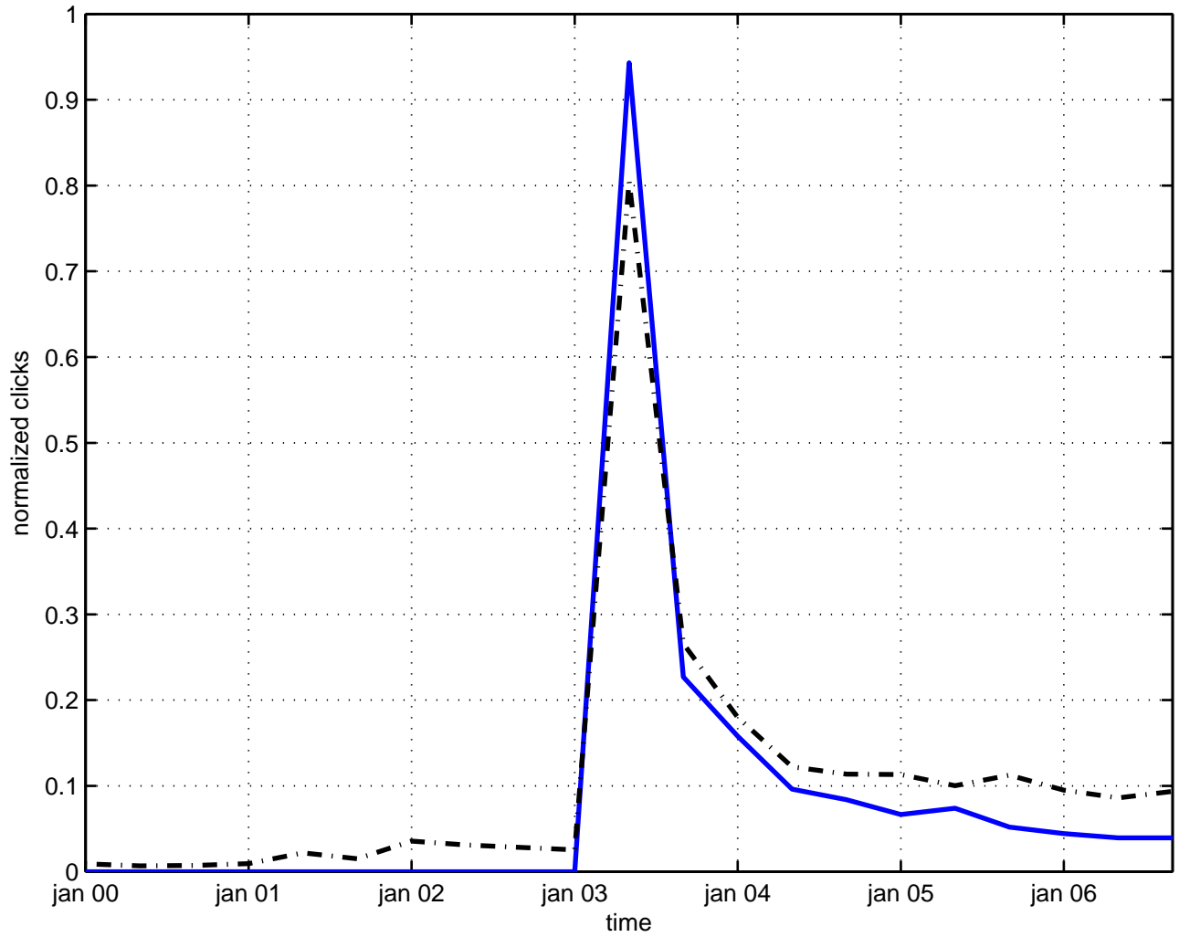
scaling symmetry breaking
