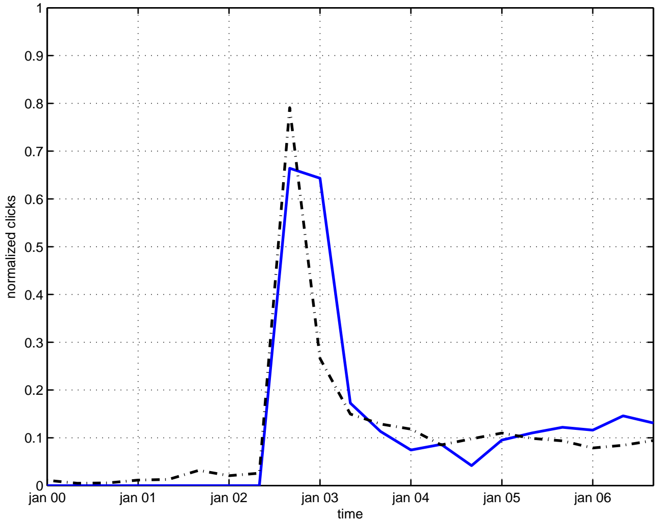
scaling operator
