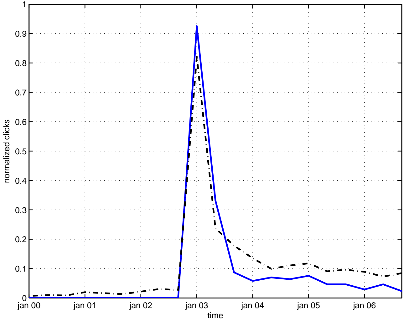
scaling network
