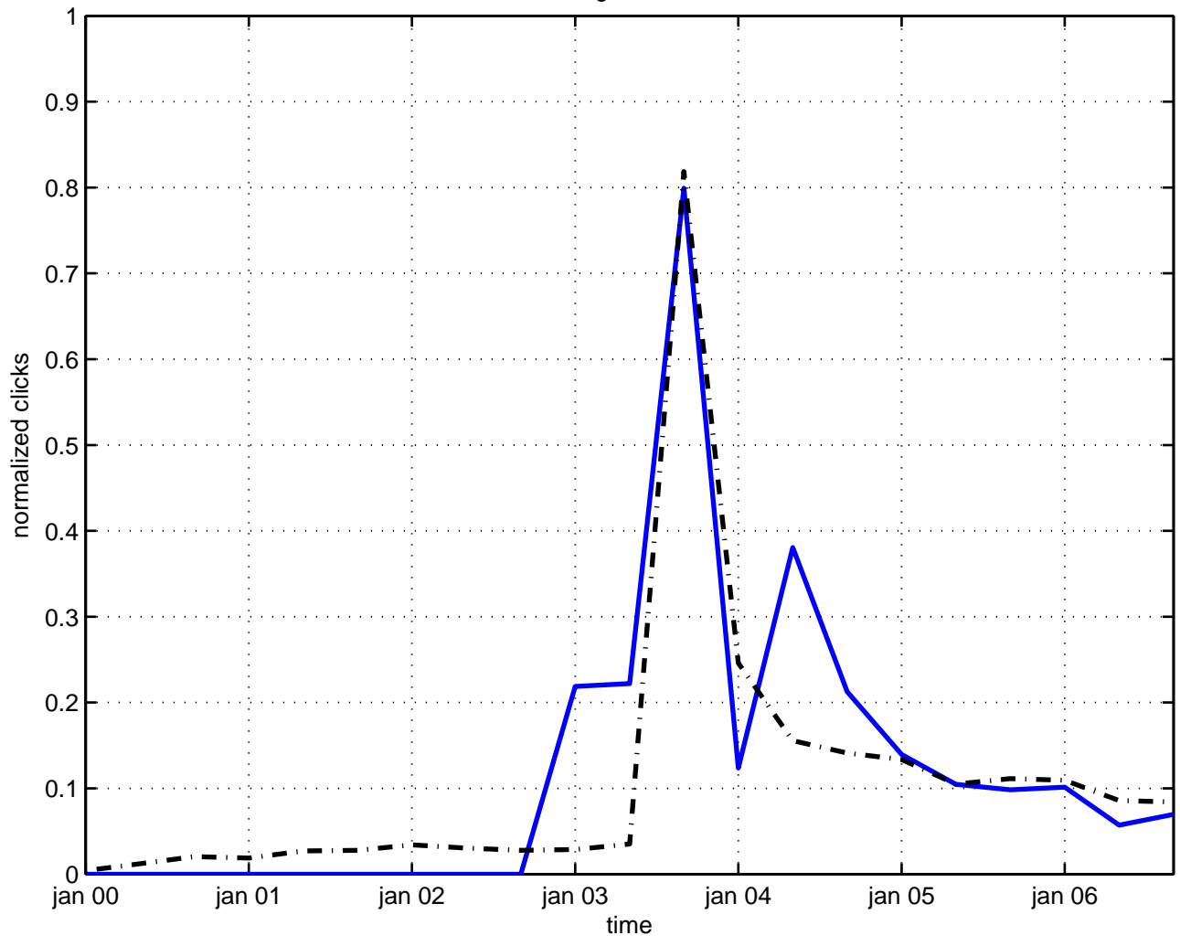
scaling invariance
