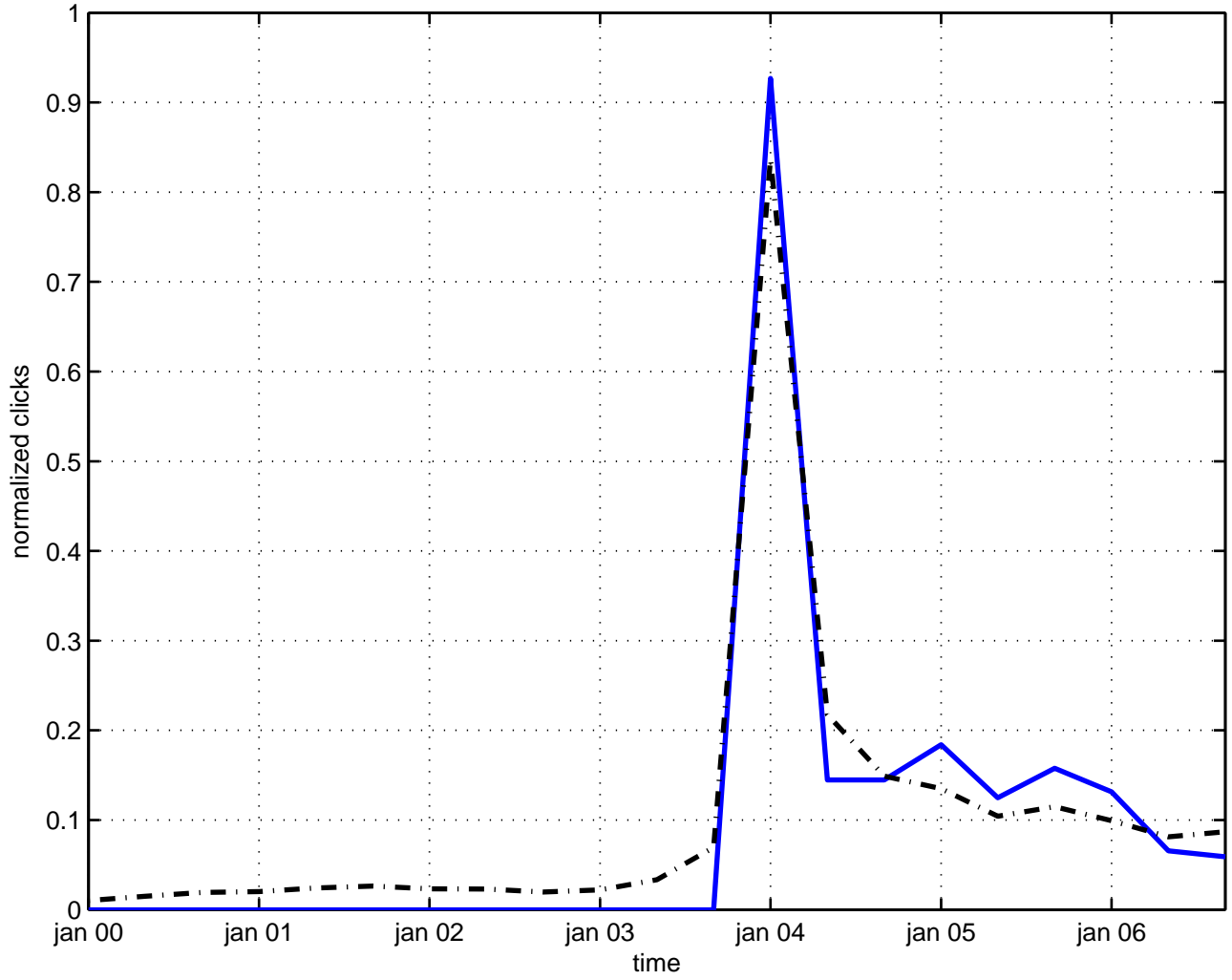
scaling fluctuation
