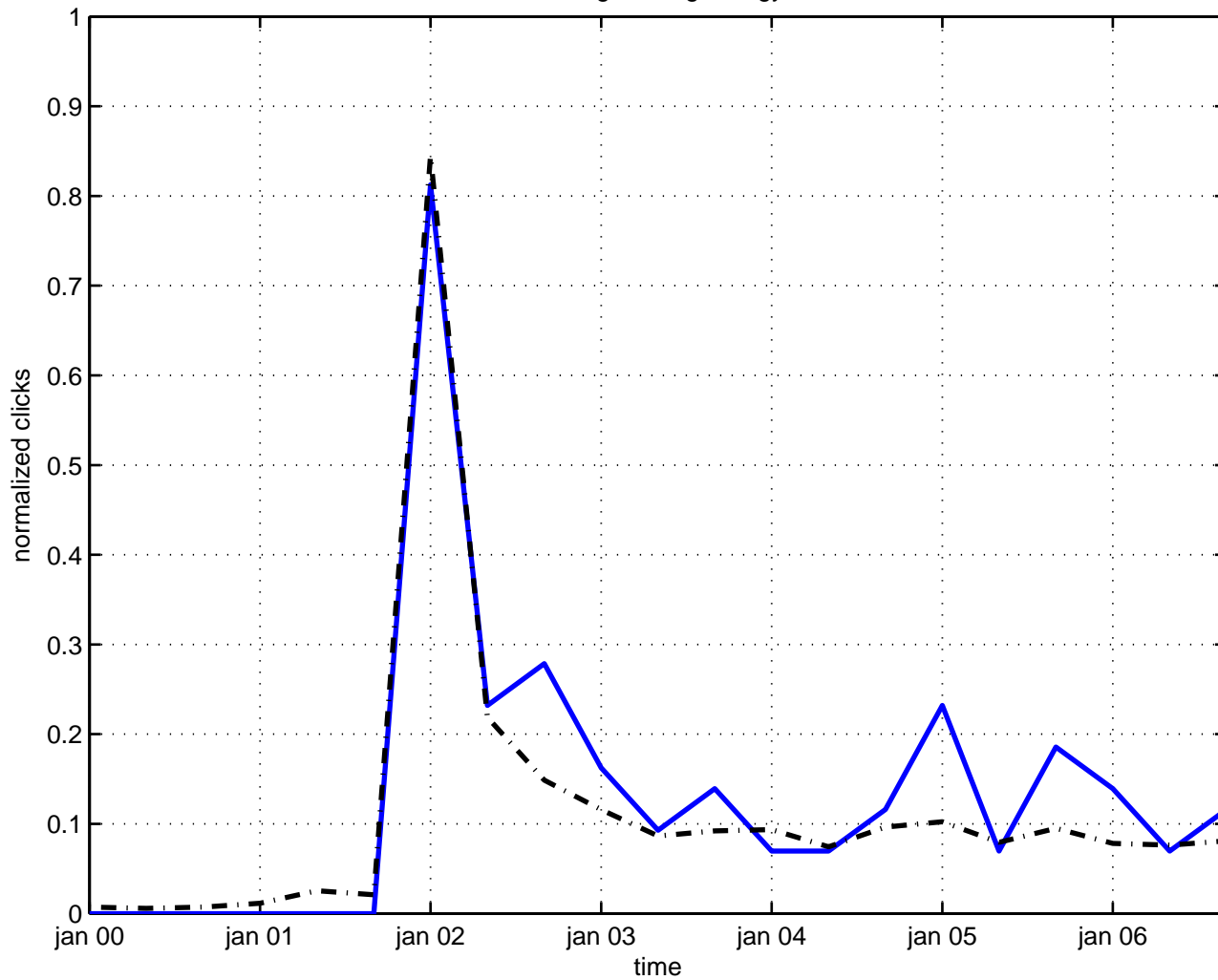
scaling binding energy
