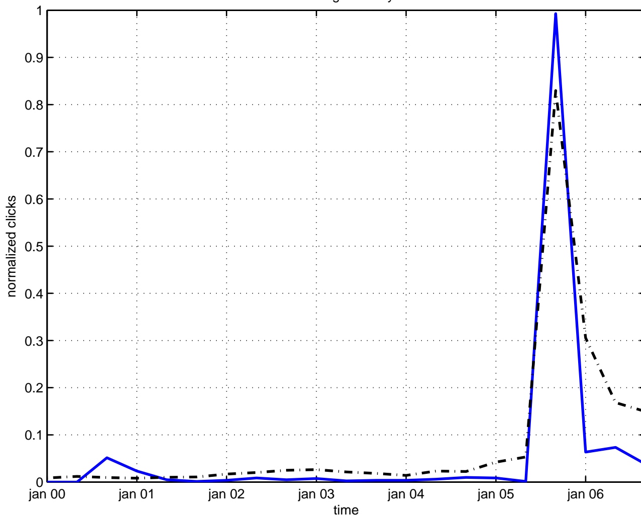
scaling anomaly
